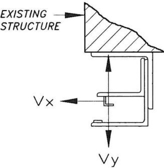
LOAD DIAGRAM
